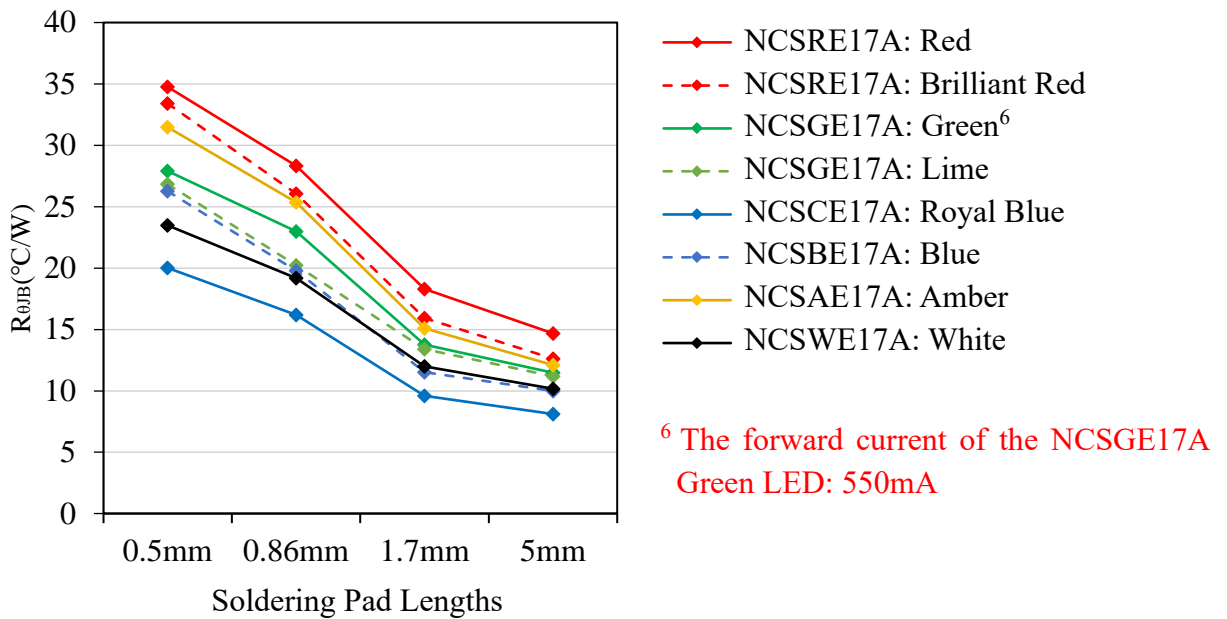
Figure 6. Thermal Resistance ( R_{\theta JB} ) of the NCSx17A LEDs on Aluminum PCBs (Thermal Conductivity of the Insulating Layer: 1.8W/m·K) at I_F=700mA^6
